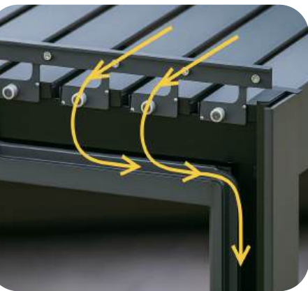
Hidden drainage system
